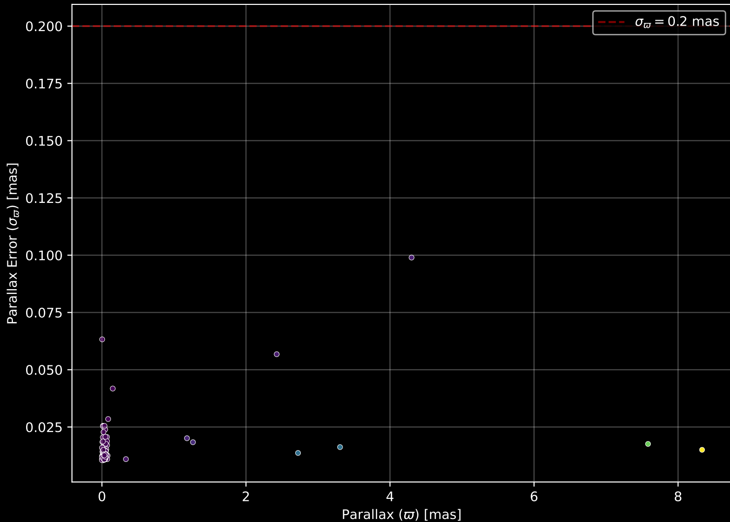
APOGEE DR17 Field: [277-32-O] Parallax Quality (n= 91)
