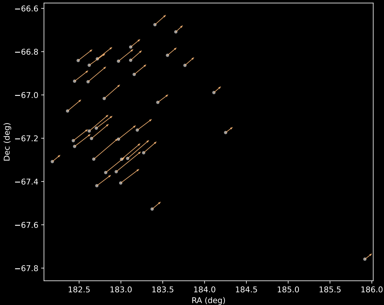
APOGEE DR17 Cluster 3 Proper Motion Vectors (n=36)
