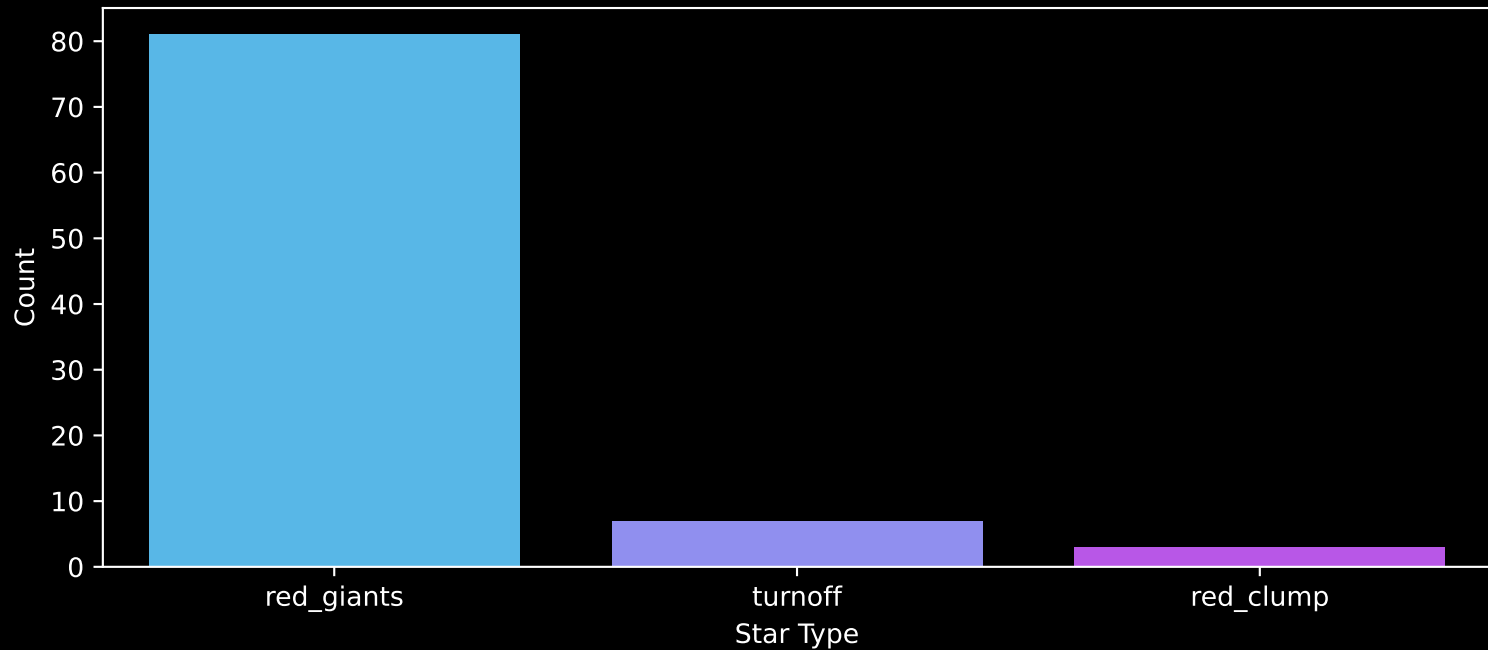
APOGEE DR17 Field: [277-32-O] Count plot of Star Type
