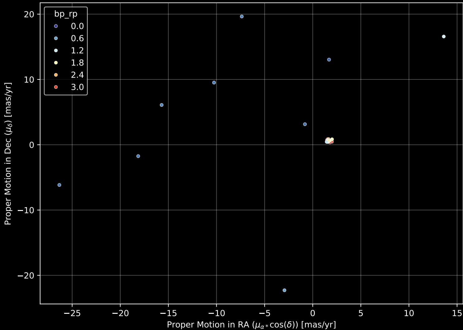
APOGEE DR17 Field: [277-32-O] Proper Motion Diagram (n= 91)
