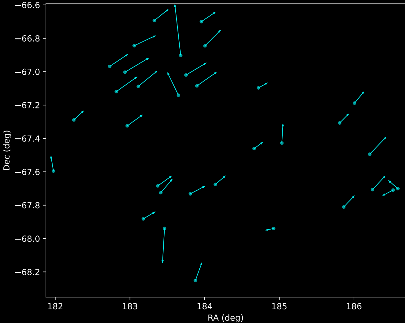
APOGEE DR17 Noise Stream Proper Motion Vectors (n=33)
