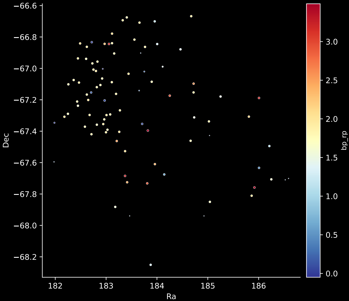
APOGEE DR17 Field: [277-32-O] Stars: 91
