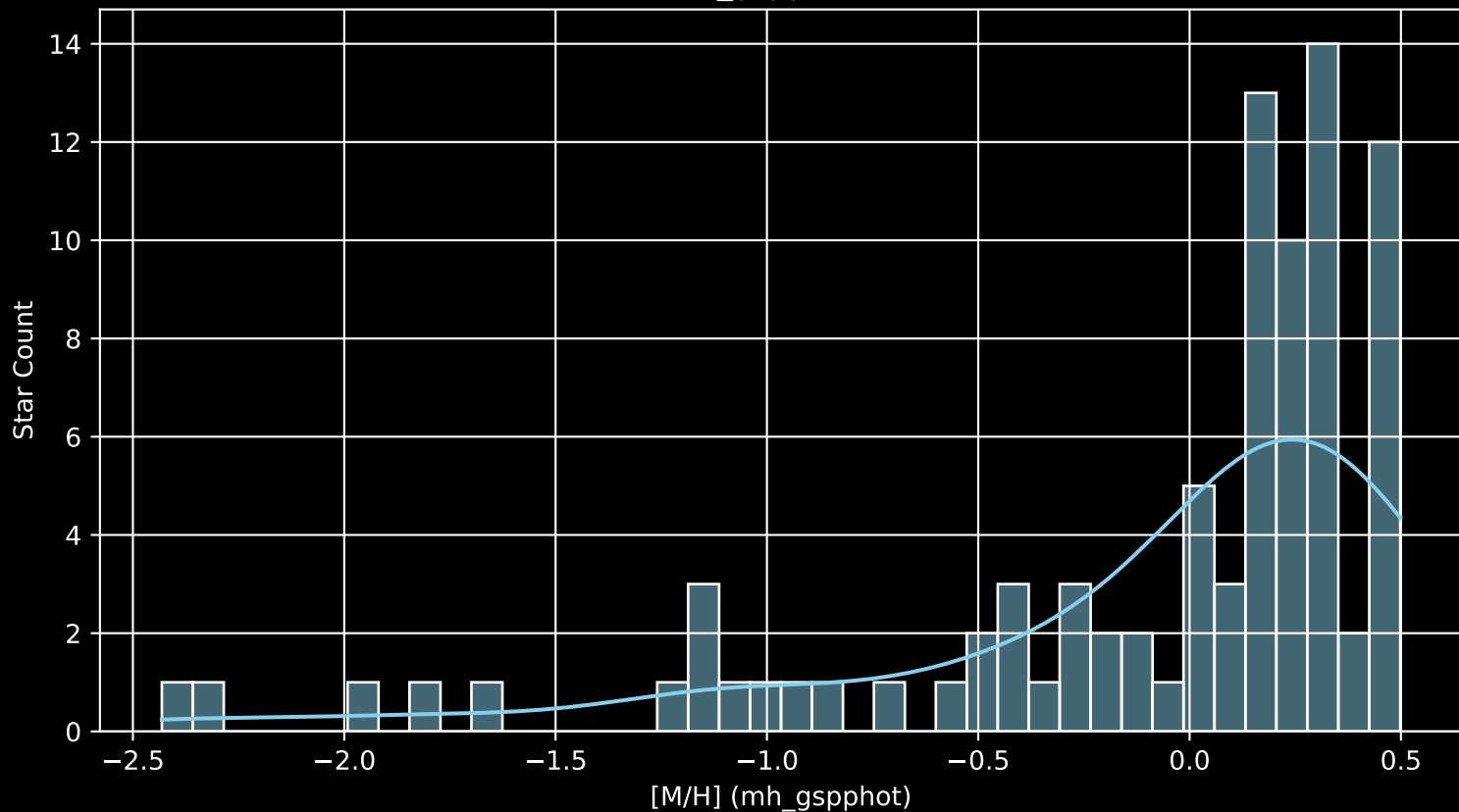
APOGEE DR17 Field: [277-32-O [M/H] (mh_gspphot) (n= 88)
