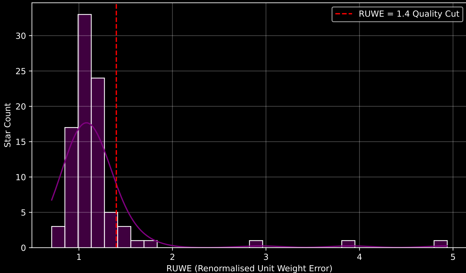
GAPOGEE DR17 Field [277-32-O] RUWE Distribution (n= 90)
